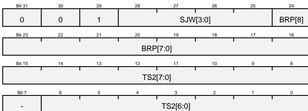
Figure 44: Structure of baud rate register dwBaudrate for USB-CANmodul1 C Rev.01
