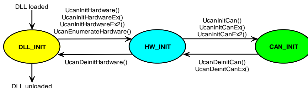
Figure 34: Software State Diagram
